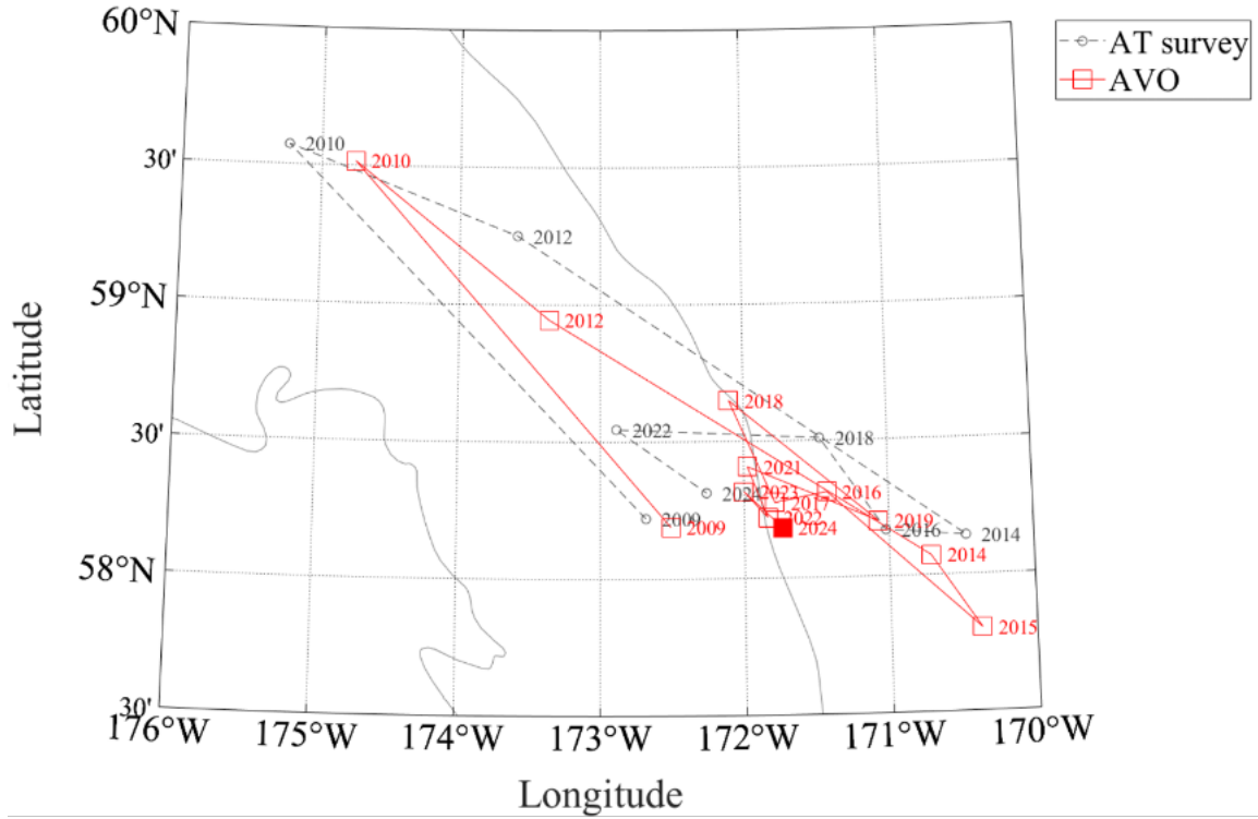
Figure 24: Geographic center of gravity estimates derived from pollock sA (m2 nmi-2) from acoustic-trawl (AT) survey (gray circles) and the acoustic vessel-of-opportunity index (red squares). The point with a filled red square is to highlight the new AVO estimate (2024). The 100 and 200 m bathymetric contours are indicated in gray. The 2018 AT survey did not complete the last 3 transects (i.e., the western-most transects) due to vessel mechanical problems, and the omission of sA from this area will bias the 2018 AT data point to the southeast.
