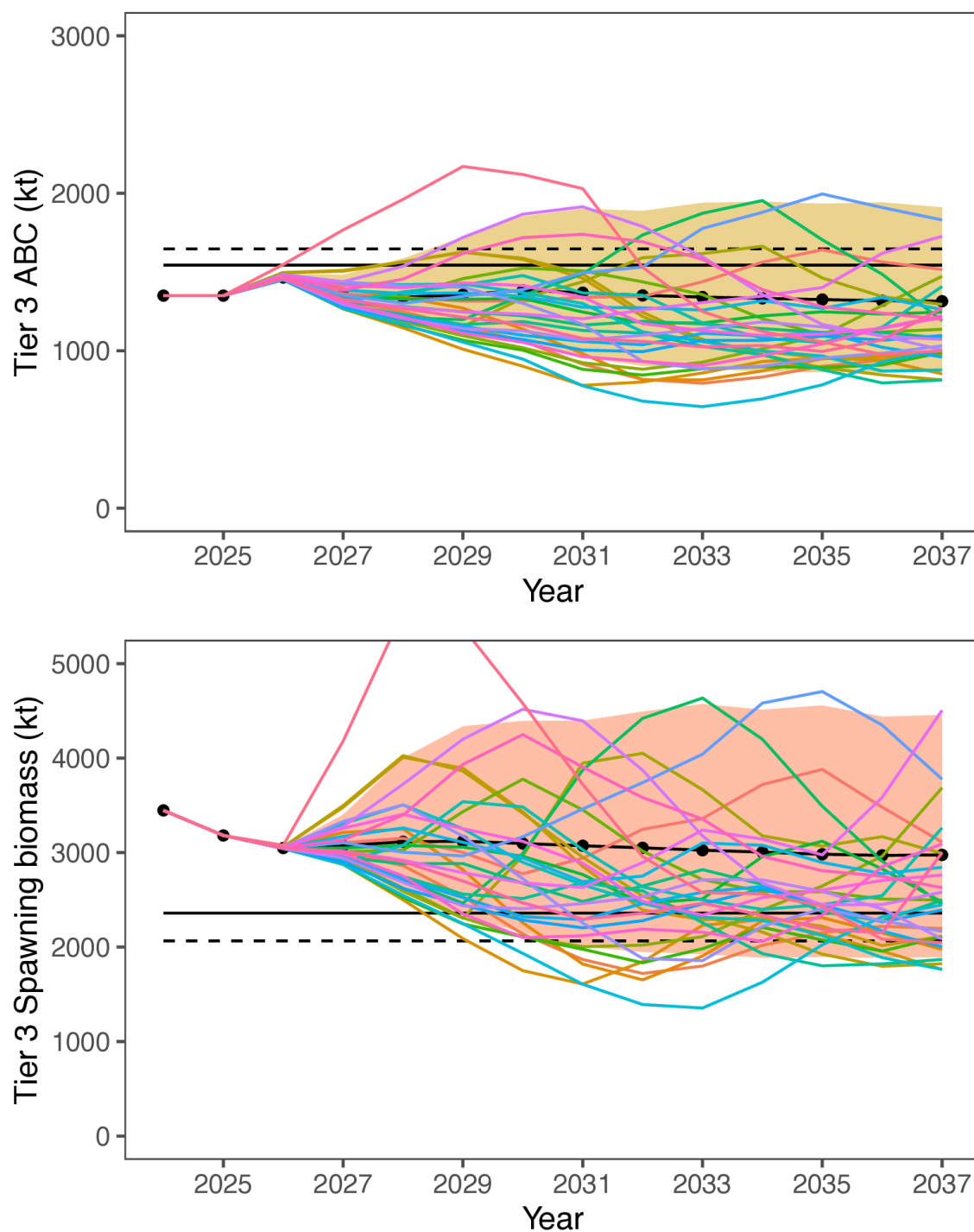
Figure 73: Projected pollock yield (top) and female spawning biomass (bottom) under Alternative 3—fishing under the recent 5-year average fishing mortality. The long-term expected values under F_{35\%} and F_{40\%} (horizontal lines) B_{40\%} are computed from average recruitment from 1978–2020.
