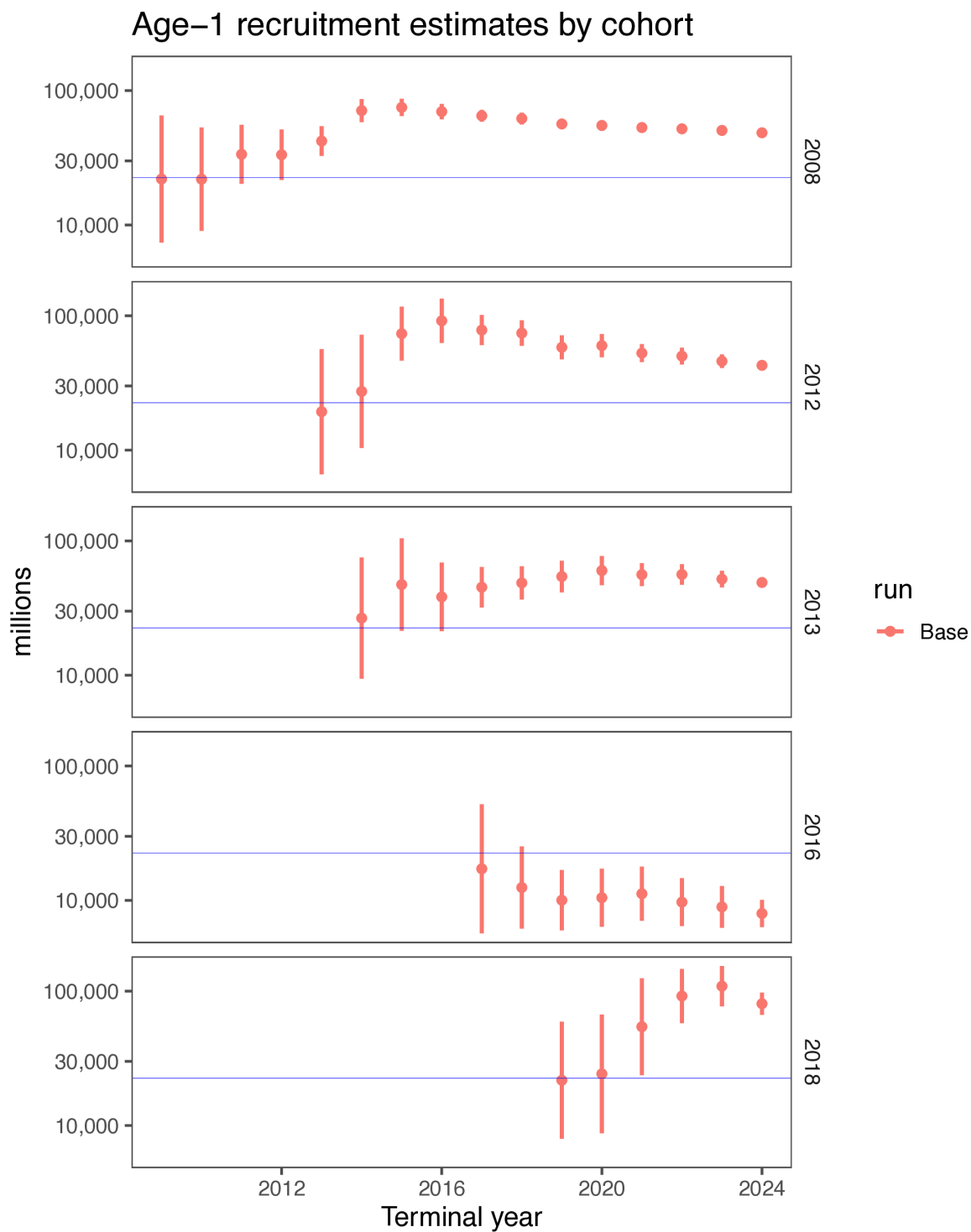
Figure 56: Retrospective evolution of EBS pollock selected year-class estimates as a function of the terminal year of data used in the model (based on retrospectives of Model 23.0).
