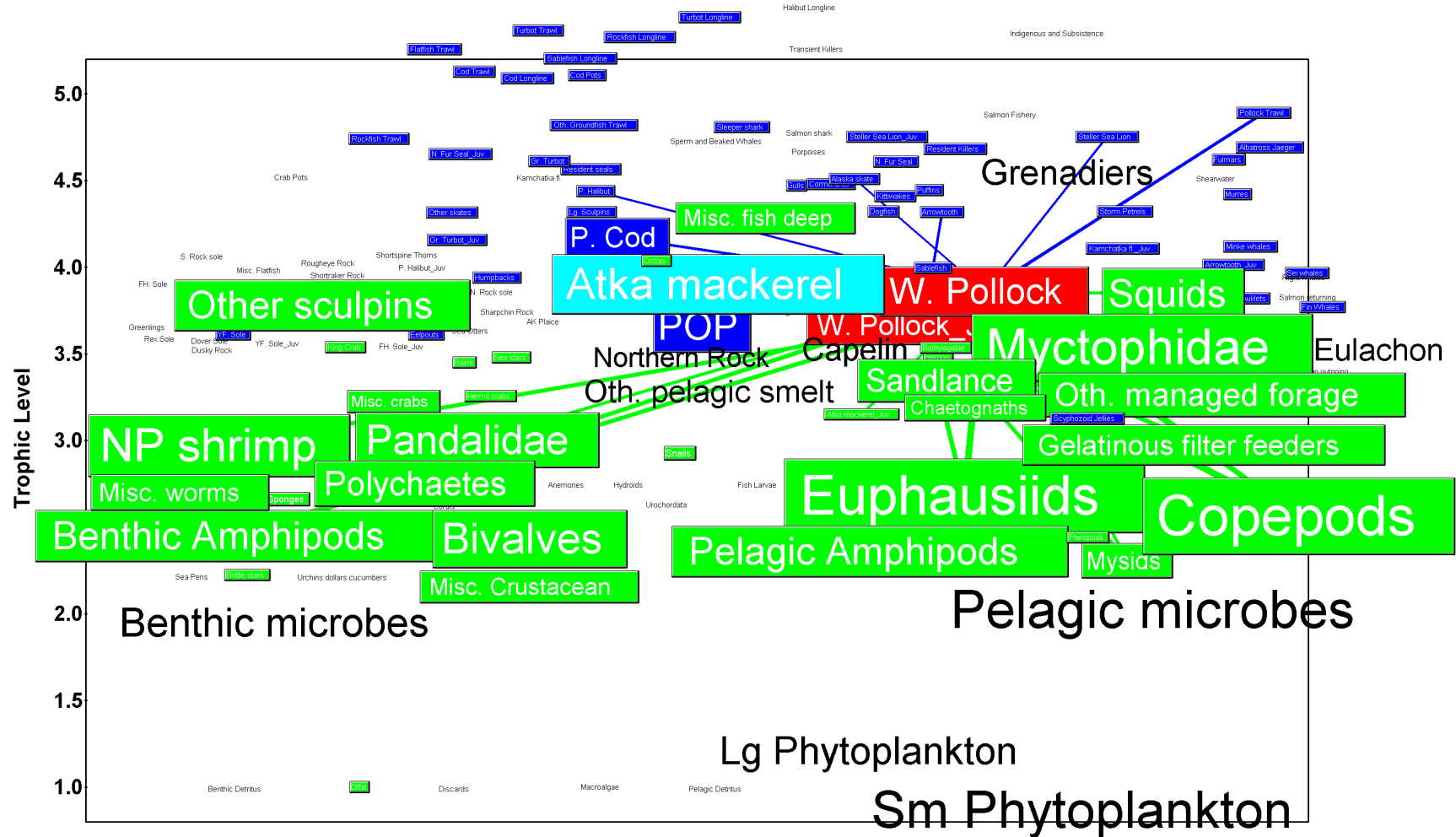
Figure 1A. 32 Adult and juvenile pollock (highlighted in red) in the AI food web (Aydin et al 2007). Predators of pollock are dark blue, prey of pollock are green, and species that are both predators and prey of pollock are light blue. Box size is proportional to biomass and lines between boxes represent the most significant energy flows.
