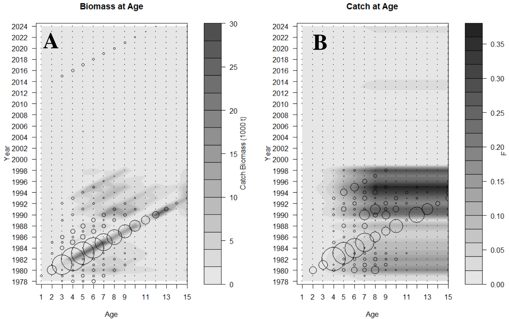
Figure 1A. 19 AI pollock authors' preferred Model 15.1 (A-contour) catch biomass in 1,000s of tons and (A-bubbles) total biomass and (B-contour) fishing mortality rates and (B-bubbles) catch biomass by age. Total biomass is scaled to 1/20th of the catch biomass in the bubble plots.
