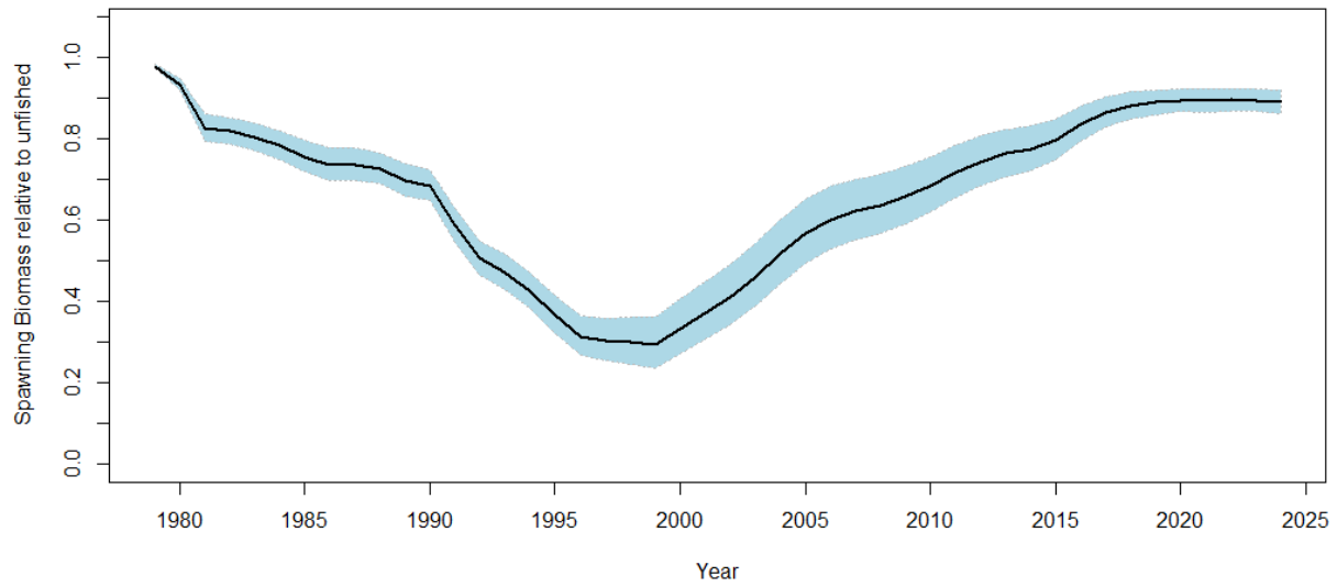
Figure 1A. 23 Aleutian Islands pollock ratio of spawning biomass with fishing relative to spawning biomass without fishing for the authors' preferred model with 95% confidence interval.
