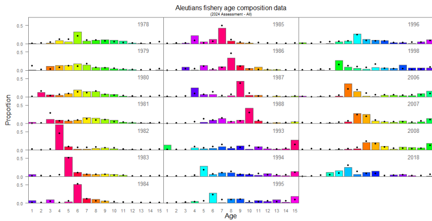
Figure 1A. 12 Model 15.1 and Model 15.2. fits to fishery age composition data for Aleutian Islands pollock. The “•” symbol are the model predictions and columns are the observed proportions at age (with colors corresponding to cohorts).
