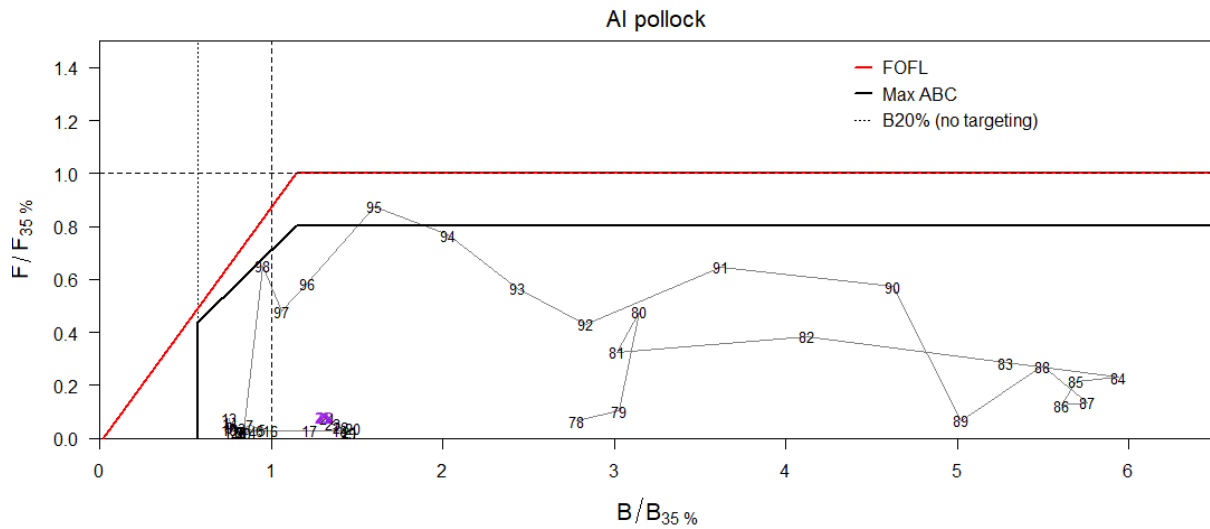
Figure 1A. 22 Aleutian Islands pollock spawning biomass relative to B_{msy} and full-selection fishing mortality relative to F_{msy} (1978-2026). The ratio of fishing mortality to F_{msy} is calculated using the estimated selectivity pattern in that year. 2025 and 2026 are plotted with catch assumed to be at the 5-year average of F = 0.032 (Alternative 3).
