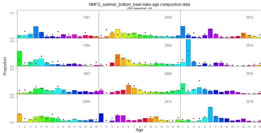
Figure 1A. 11 Aleutian Islands pollock Model 15.1 and Model 15.2 fit to NMFS summer bottom trawl survey age composition data. The “•” symbol are the model predictions and columns are the observed proportions at age (with colors corresponding to cohorts).
