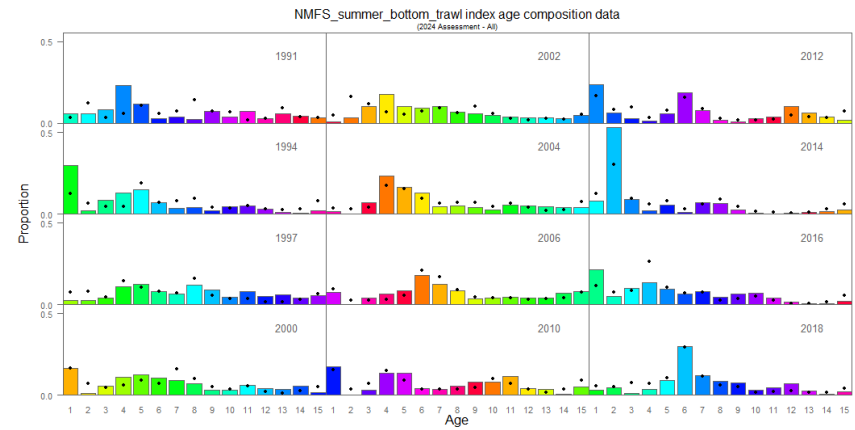
Figure 1A. 11 Aleutian Islands pollock Model 15.1 and Model 15.2 fit to NMFS summer bottom trawl survey age composition data. The “•” symbol are the model predictions and columns are the observed proportions at age (with colors corresponding to cohorts).
