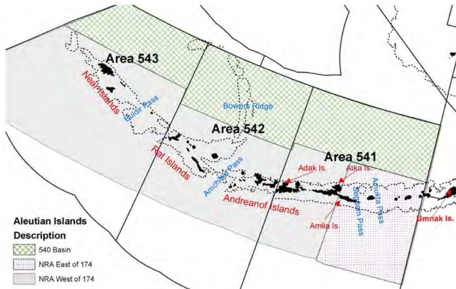
Figure 1A. 3 Regions defined for consideration of alternative data partitions for Aleutian Islands Region pollock. The abbreviation “NRA” represents the Near, Rat, and Andreanof Island group. There are no models for 2018 that consider the NRA east-west partition at
