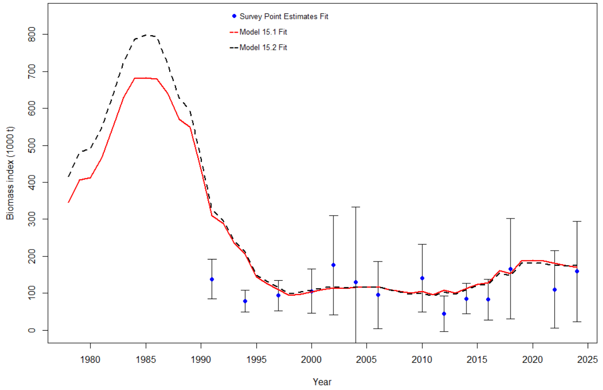
Figure 1A. 10 Model fits to NMFS summer bottom trawl survey.
