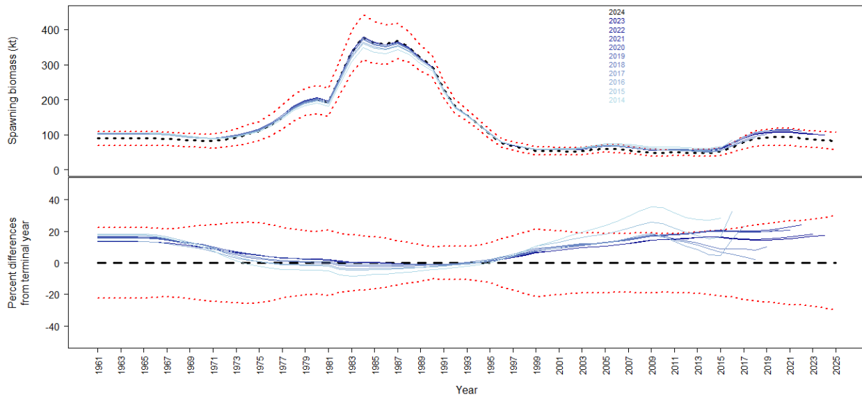
Figure 1A. 24 Retrospective analysis for Authors' preferred Model 15.1 with data for the previous 10 years being systematically removed from the model. Black dashed line is the 2024 Model 15.1 estimate, the red dotted lines are the 95% confidence intervals calculated as \pm 1.96 \times standard deviation.
