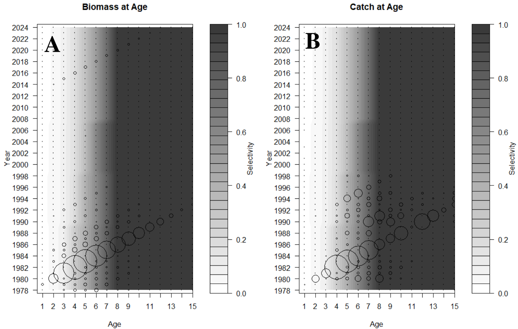
Figure 1A. 20 Contour plots of fishery selectivity by age for AI pollock with bubble plots of (A) total biomass at age and (B) catch biomass at age for the Authors' preferred Model 1.0. Total biomass is scaled to 1/20 of the catch biomass bubbles.
