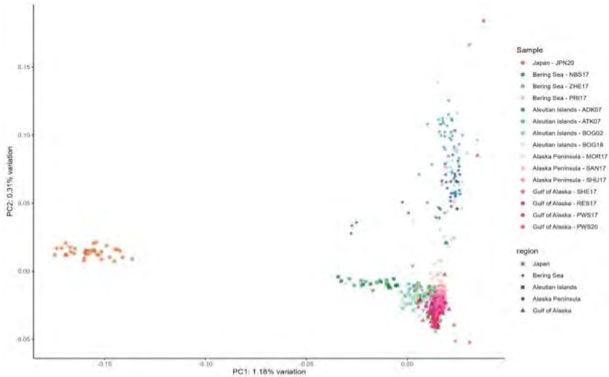
Figure 1A. 2 Principal component analysis analyzing the ~2 million polymorphic loci found in our sample set throughout the walleye pollock genome.
