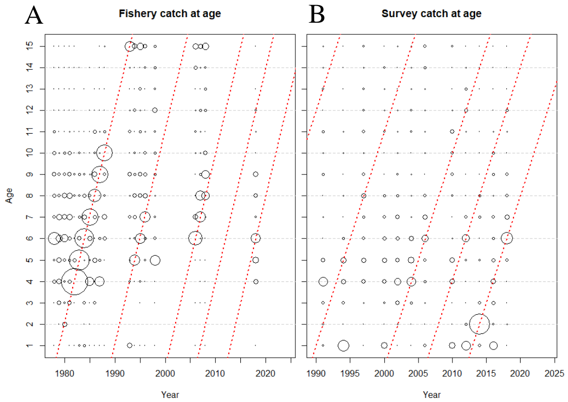
Figure 1A. 5 Age distributions for 1978-2024 Aleutian Islands pollock fishery (A; left) and 1991 - 2024 Aleutian Islands Bottom Trawl surveys (B; right). The 1978, 1989, 2000, 2006, and 2012-year classes are indicated by the diagonal dashed lines.
