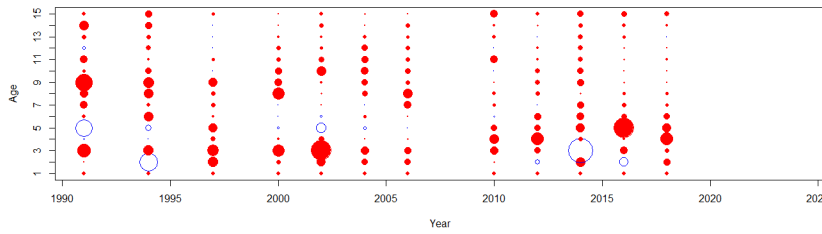
Figure 1A. 14 Standardized residuals for fits to the fishery (top) and survey (bottom) proportion-at-age data for AI pollock Model 15.1 and Model 15.2. Red indicating positive residuals and blue negative residuals.
