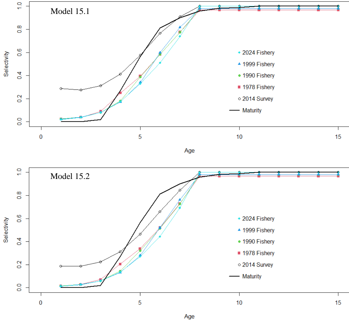
Figure 1A. 15 Fishery and survey selectivity estimates with maturity at age for Aleutian Islands pollock models.
