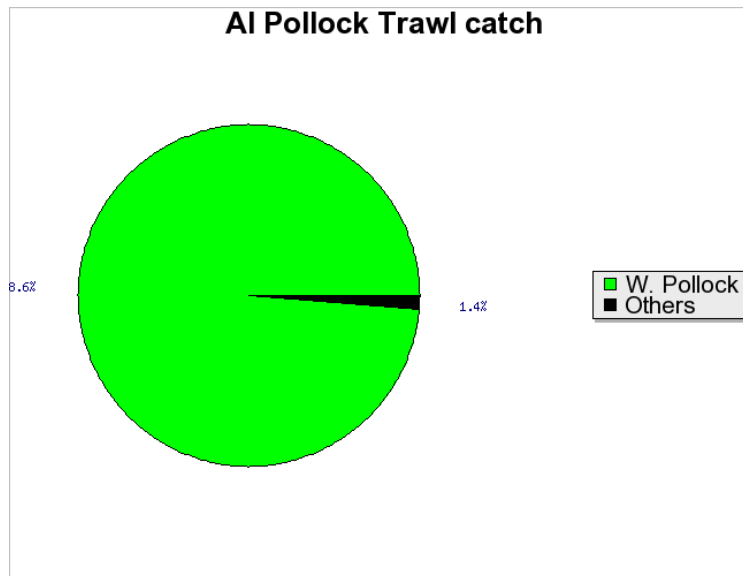
Figure 1A. 31 Catch composition of the AI pollock trawl fishery during the early 1990's, as used in the food web model (Aydin et al. 2007).
