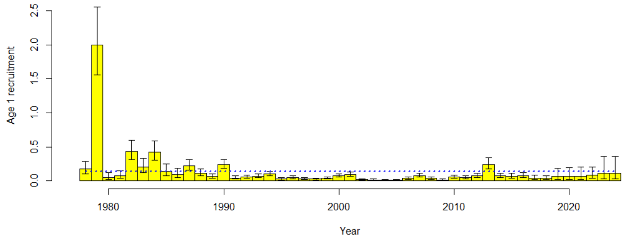
Figure 1A. 21 Authors' preferred model estimates of Aleutian Islands pollock age 1 recruitment. The vertical bars represent the upper and lower 95% confidence bounds. The dotted line is the 1978-2022 mean age-1 recruitment.
