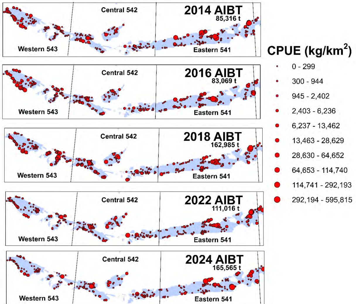
Figure 1A. 6 Catch per unit effort (kg/km 2 ) for surveys of pollock in the Aleutian Islands Region, 2014-2024. The shaded area is the Aleutian Islands shelf area less than 300m depth.
