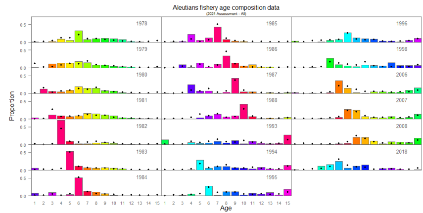
Figure 1A. 12 Model 15.1 and Model 15.2. fits to fishery age composition data for Aleutian Islands pollock. The “•” symbol are the model predictions and columns are the observed proportions at age (with colors corresponding to cohorts).
