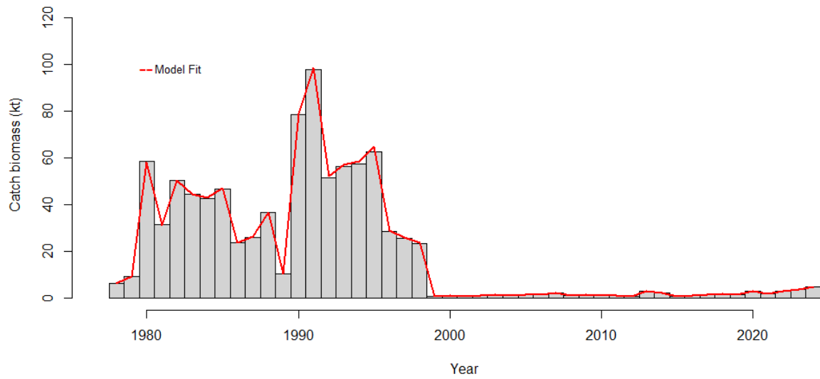
Figure 1A. 18 Fits to total catch in 1,000s of tons for AI pollock over time 1978-2024.
