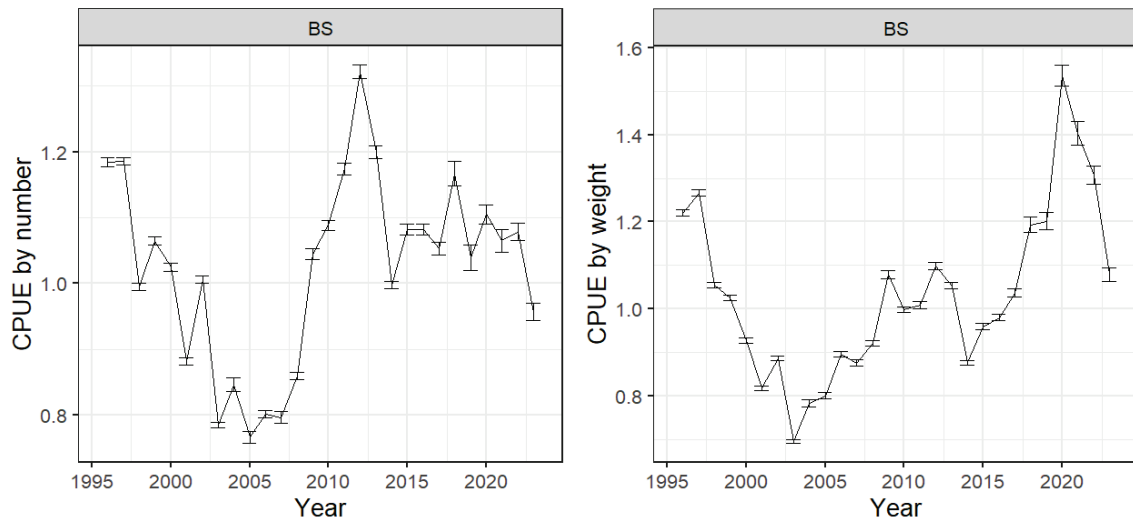
Figure 2.10. Thompson et al. (2021) combined fishery CPUE index estimates for 1996-2023 by (left) number and (right) weight of fish.
